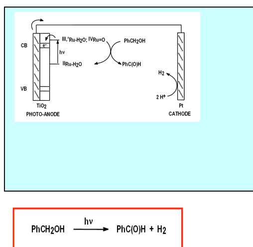
Fig. 2 - Proposed photo-oxidation scheme for organic substrates based on Ru complexes.
